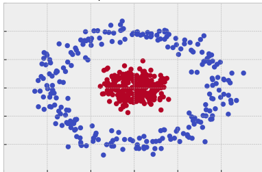
Spectral Circles
